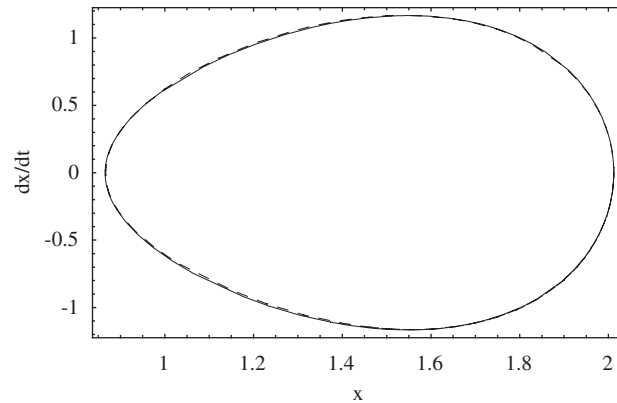
Fig. 3. Limit cycle solutions of Eq. (72) obtained analytically (—) and numerically (---).
